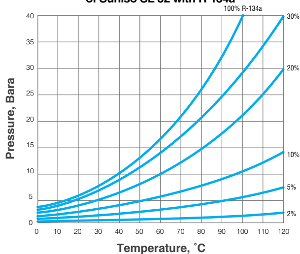
Dilution Chart of Suniso SL 32 with R-134a
